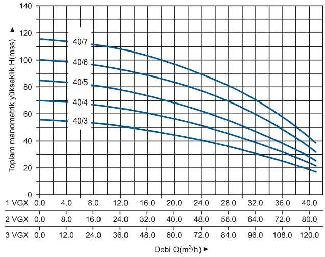
HİDROLİK PERFORMANS EĞRİSİ
