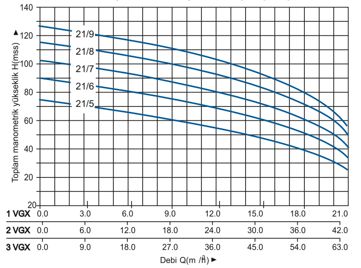
HİDROLİK PERFORMANS EĞRİSİ
