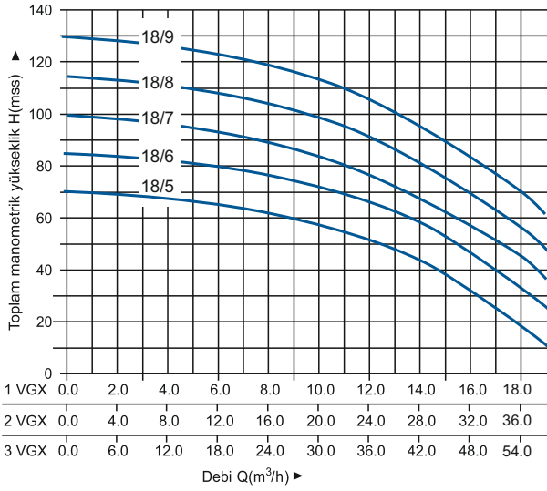
HİDROLİK PERFORMANS EĞRİSİ
