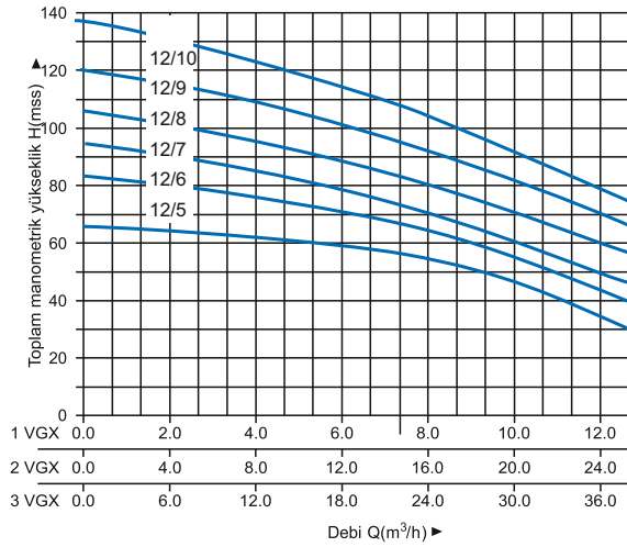
HİDROLİK PERFORMANS EĞRİSİ
