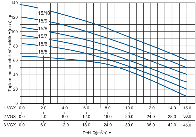
HİDROLİK PERFORMANS EĞRİSİ
