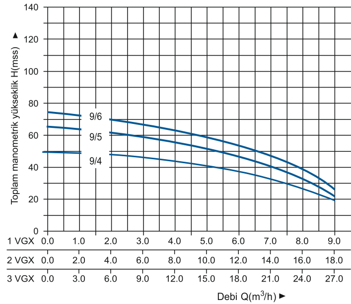
HİDROLİK PERFORMANS EĞRİSİ
