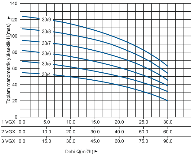
HİDROLİK PERFORMANS EĞRİSİ
