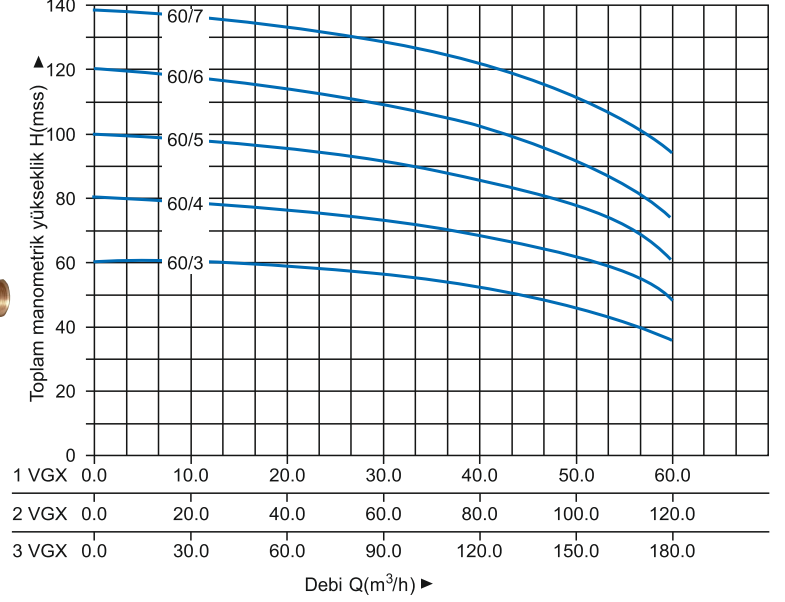
HİDROLİK PERFORMANS EĞRİSİ
